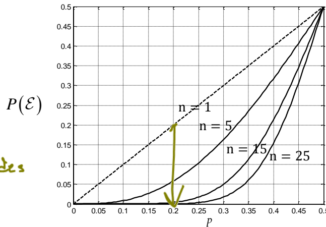
Figure 12: Bit error probability for a simple system that uses repetition code at the transmitter (repeat each bit n times) and majority vote at the receiver. The channel is assumed to be binary symmetric with bit error probability p .
